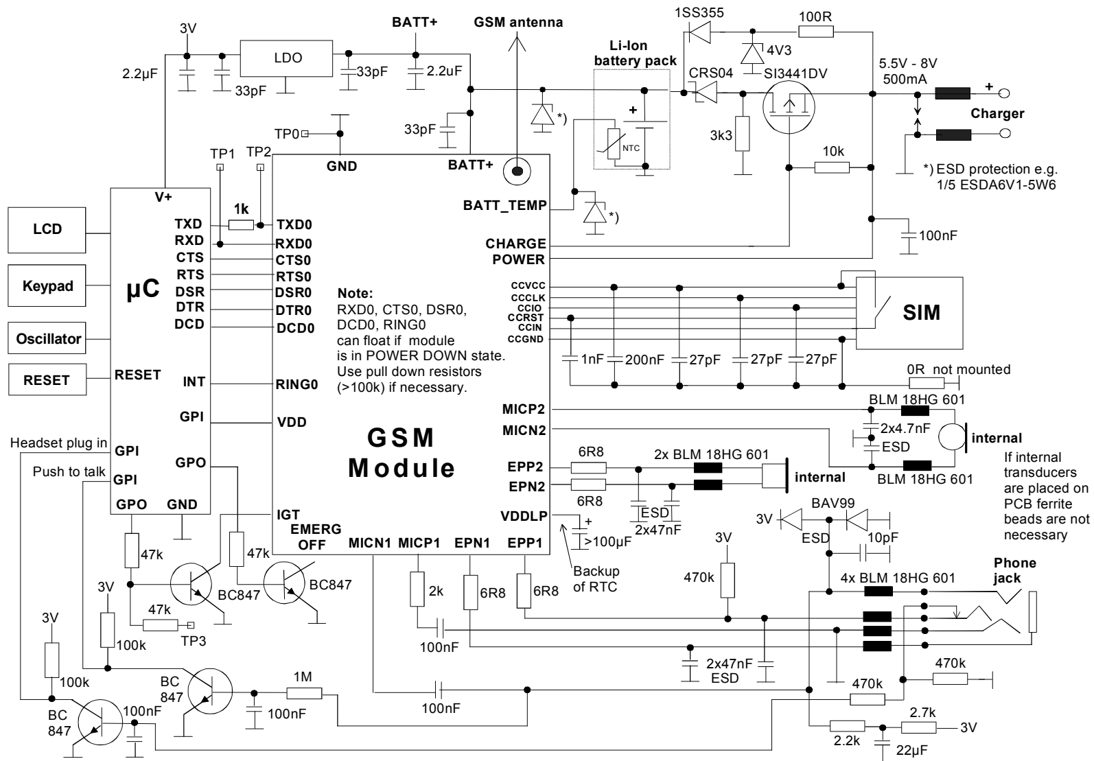
Figure 45: Schematic diagram of MC46 sample application
